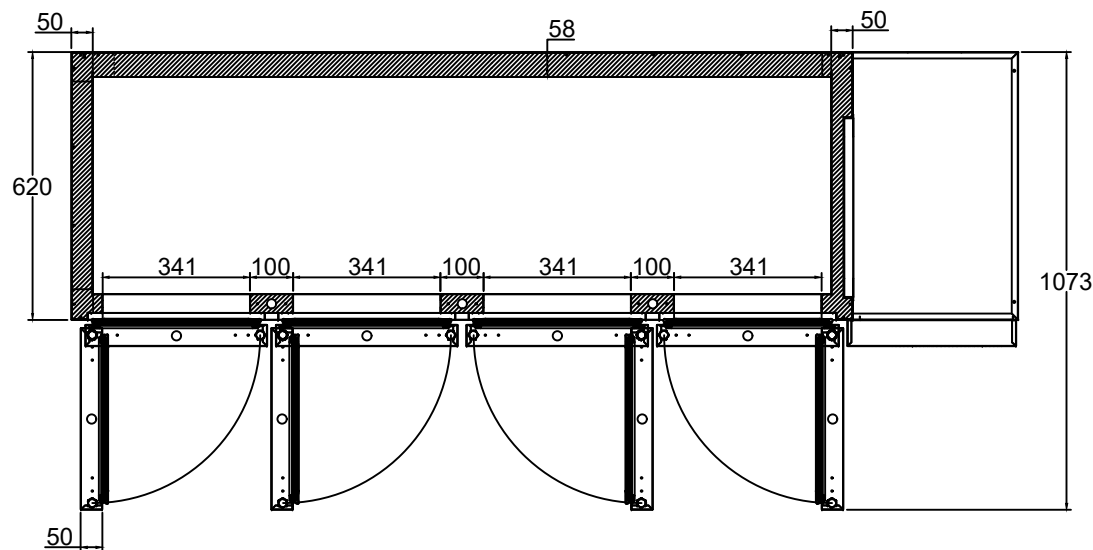
SECTION B-B
